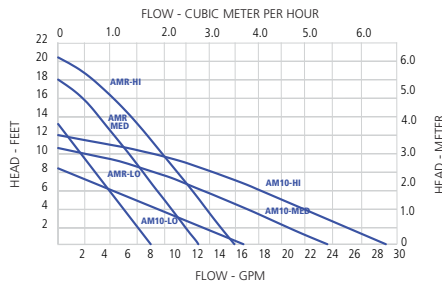
PERFORMANCE DATA 3 - Speed Curves
