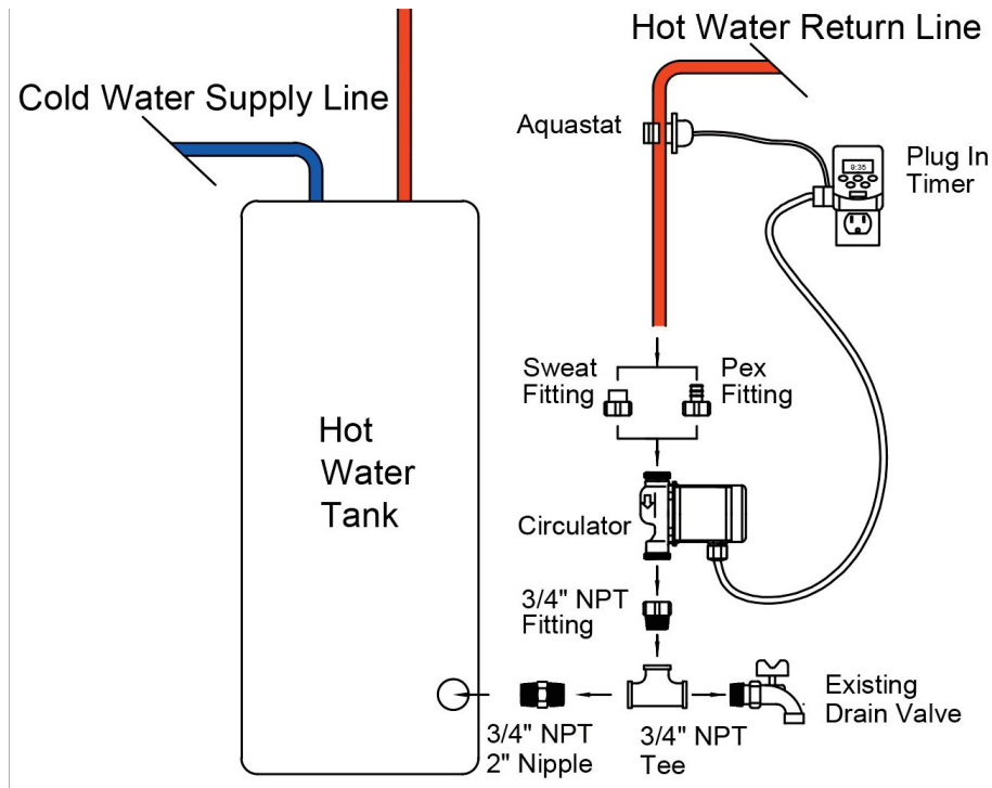
Installation Diagram AquaMotionHot Two
