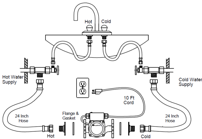
(Figure 2) AquaMotionHot One AMH3K-R (Under Sink Installation)
