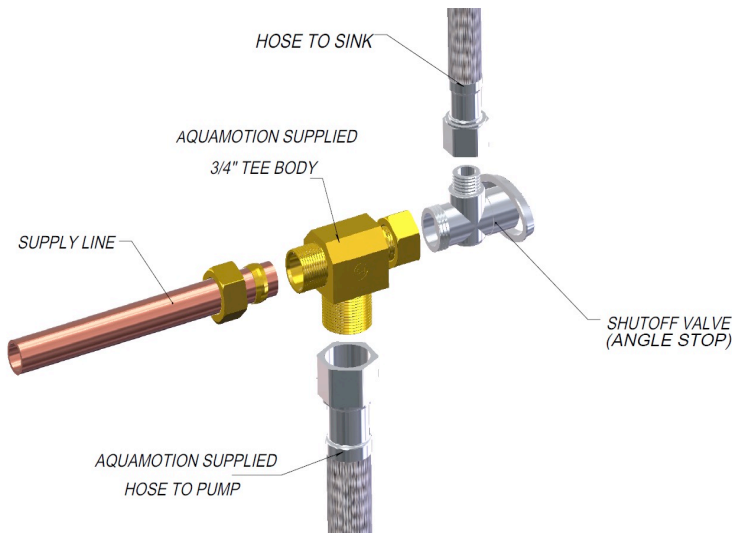
(Figure 1) Shut Off Valve Installation
