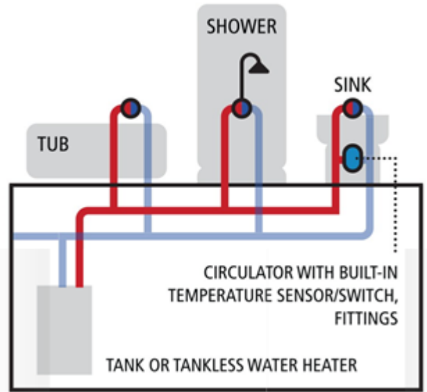
Installation Diagram AquaMotionHot One
