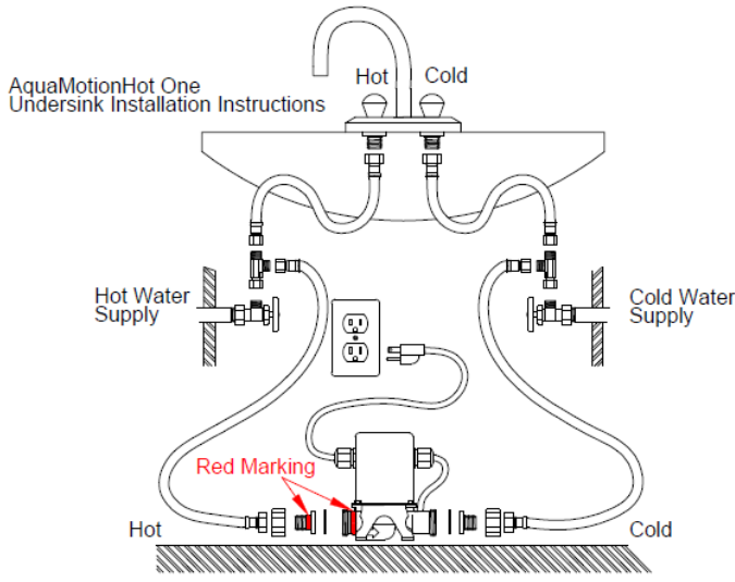
(Figure 1) AquaMotionHot One AMH1K-1 (Under Sink Installation Instructions)
