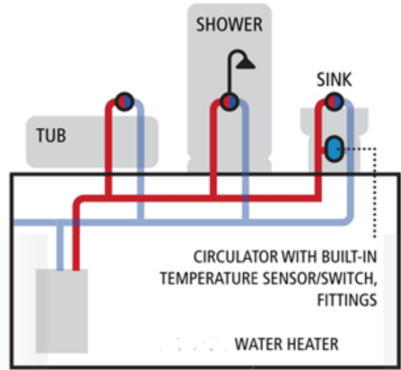
Installation Diagram AquaMotionHot One
