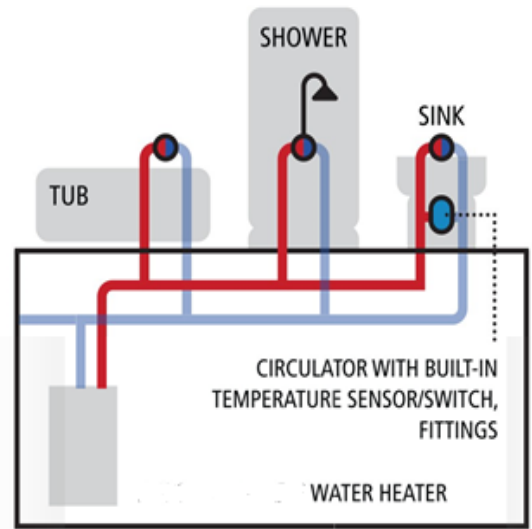
Installation Diagram AquaMotionHot One
