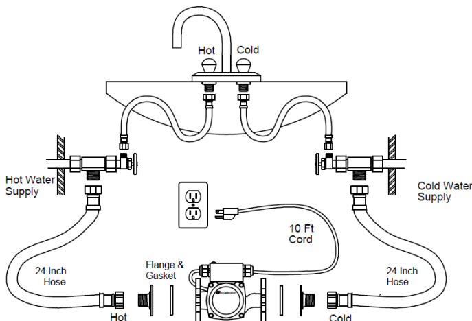
(Figure 1) Shut Off Valve Installation
