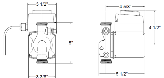
Circulator Dimensions
