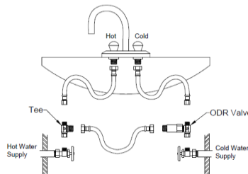
ODR Valve Installation
