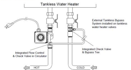
Circulator Installation
